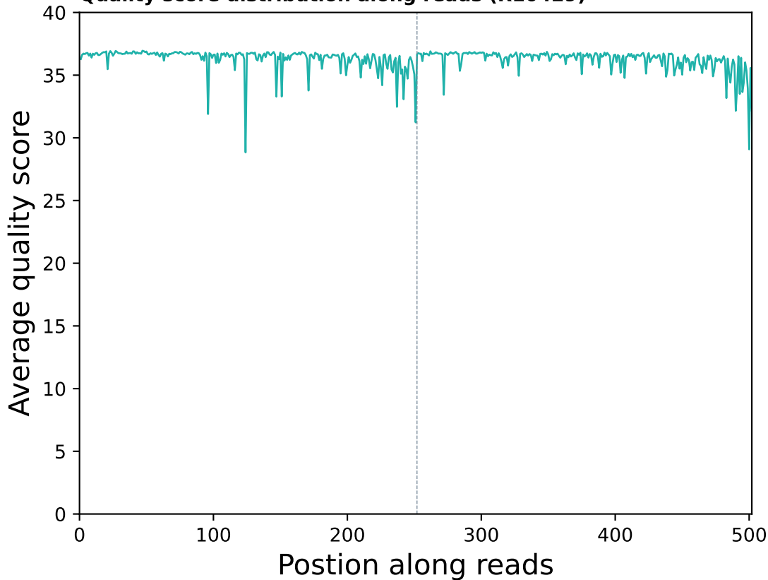
Quality score distribution along reads (R10429)
